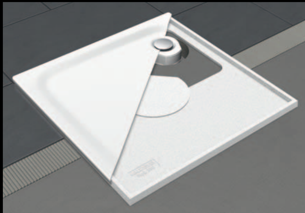
Cross section of SUPERPLAN with low profile support
